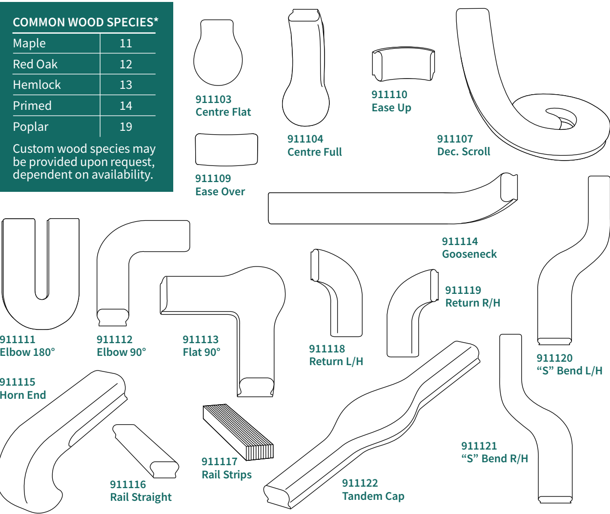
911 PROFILE
