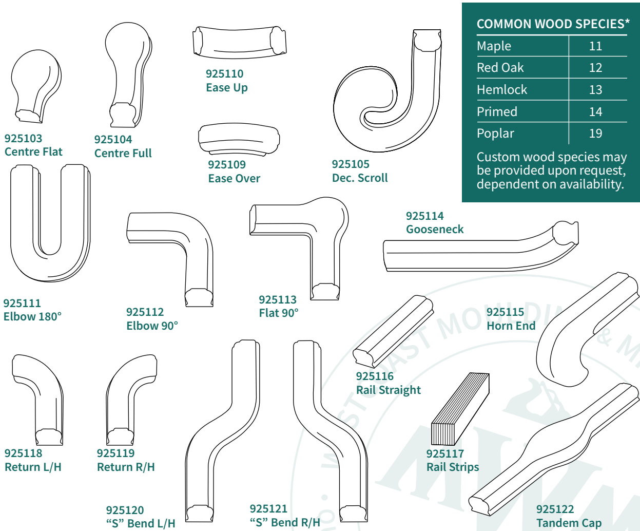
925 PROFILE
