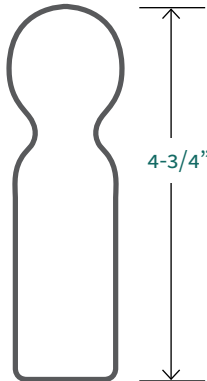
946106 Comm. Sq. Top 1-7/16" x 4-3/4"
