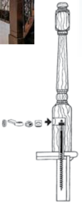
975116 Quick Mount Bolt Kit 11" Lag Bolt, 1 Curved Washer, 1 Nut, 1-1/2" Tapered Plugs
